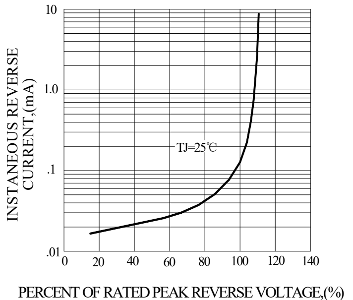
FIG.4-TYPICAL REVERSE CHARACTERISTICS
